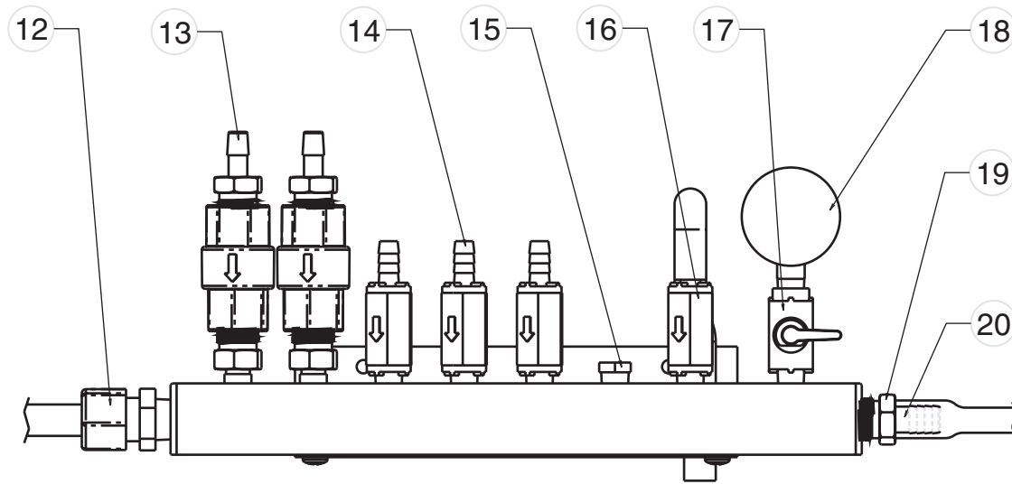
Figure 4.0.c Manifold
