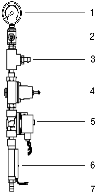
Figure 4.0.a Industrial Flush Valve
