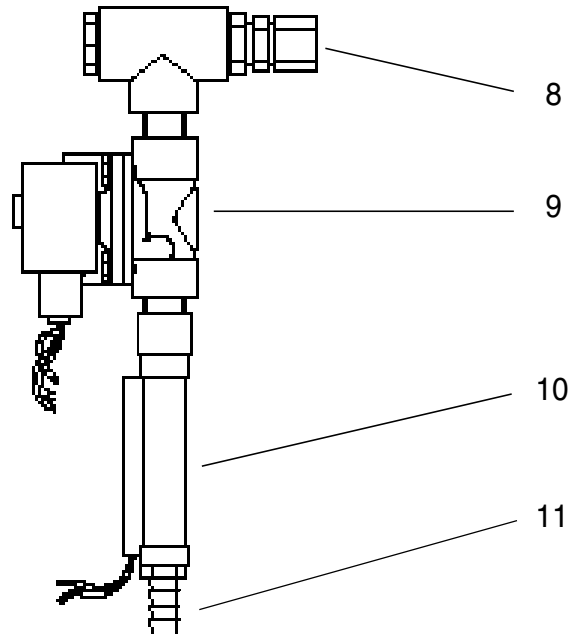
Figure 4.0.b Standard Flush Valve
