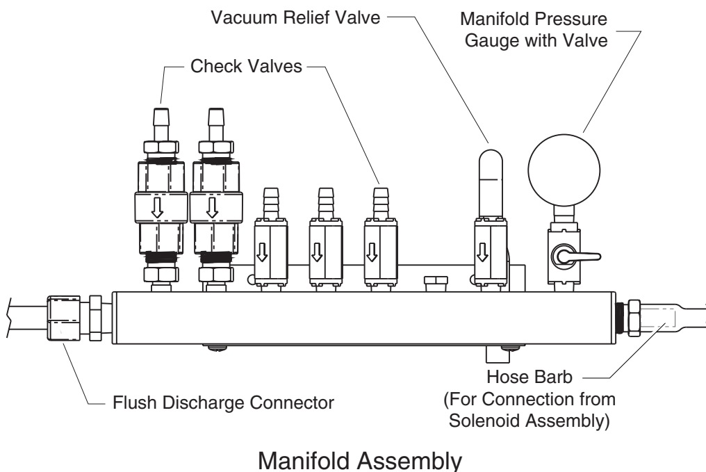
Figure 1.0.c Description, Manifold
