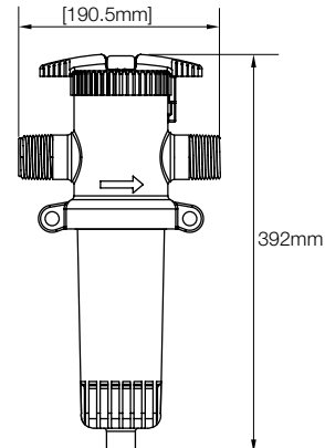
1.5" Filter dimensions
